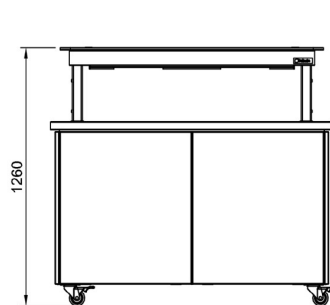
Front Elevation
