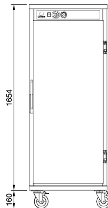
Front Elevation
